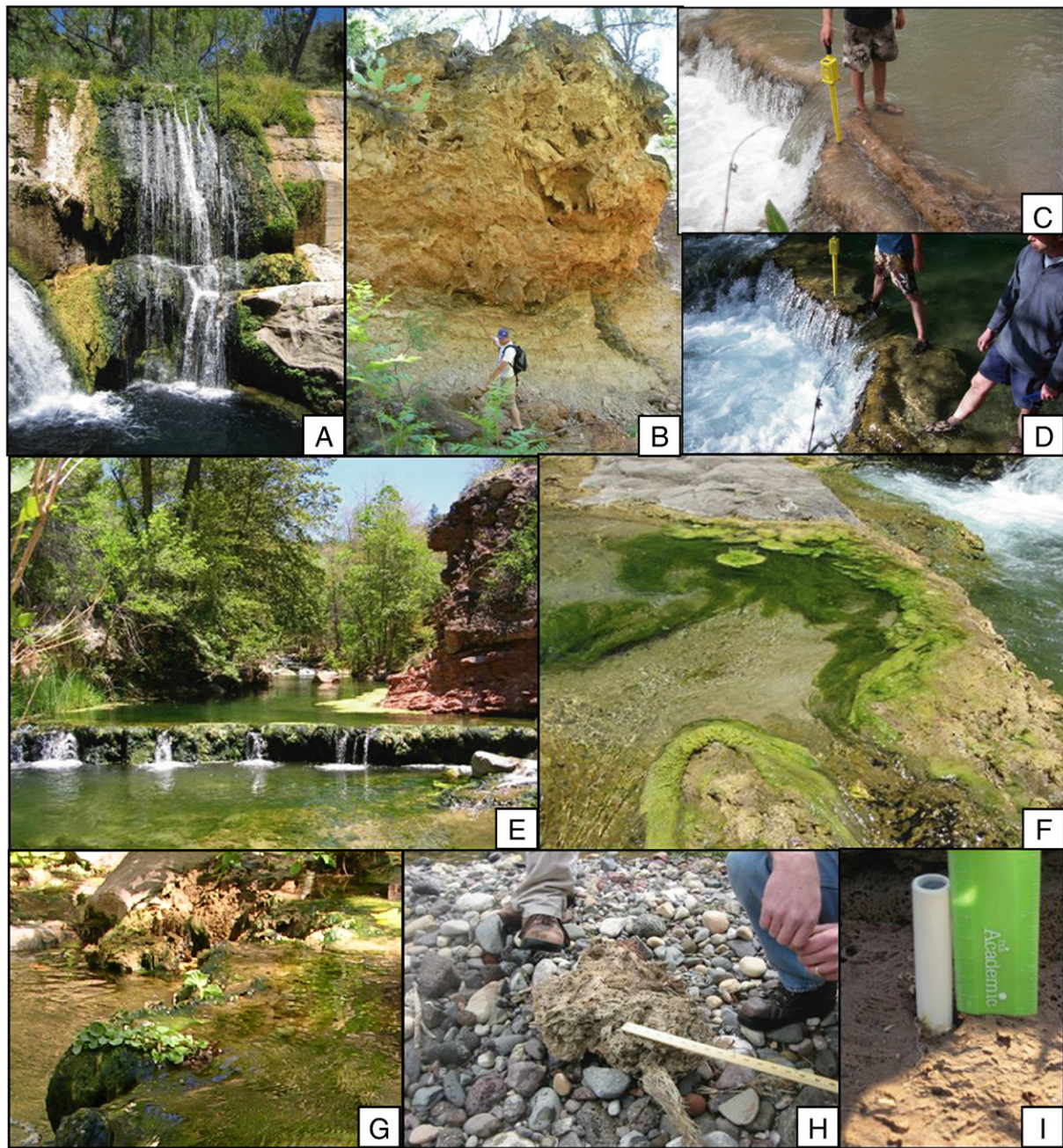
Fig. 3. Photographs. A) Fossil Creek diversion dam (~8 m in height), B) relict pre-diversion travertine structure, C) travertine dam prior to trapping large woody debris (LWD), and D) same dam 1 year later with trapped LWD, E) channel-spanning travertine dam (crest ~50 cm above downstream water surface), F) algae trapped on dam crest (water flows left to right; photo foreground spans ~3 m), G) macrophytes (~5 cm in height) colonizing travertine dam surface, flow is from right to left, H) travertine eroded in winter flood from an actively forming dam, I) magnet housing tube exposed by erosion (protruding ~7 cm).
