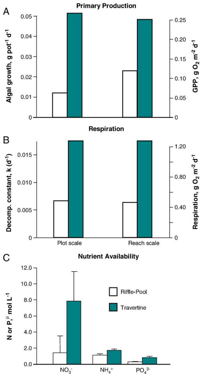
Fig. 5. Ecosystem response to travertine morphology. Compared to non-travertine riffle-pool morphology downstream on Fossil Creek, travertine dams enhance: A) primary productivity, B) respiration, and C) nutrient availability (modified from Marks et al., 2006; Carter and Marks, 2007).
