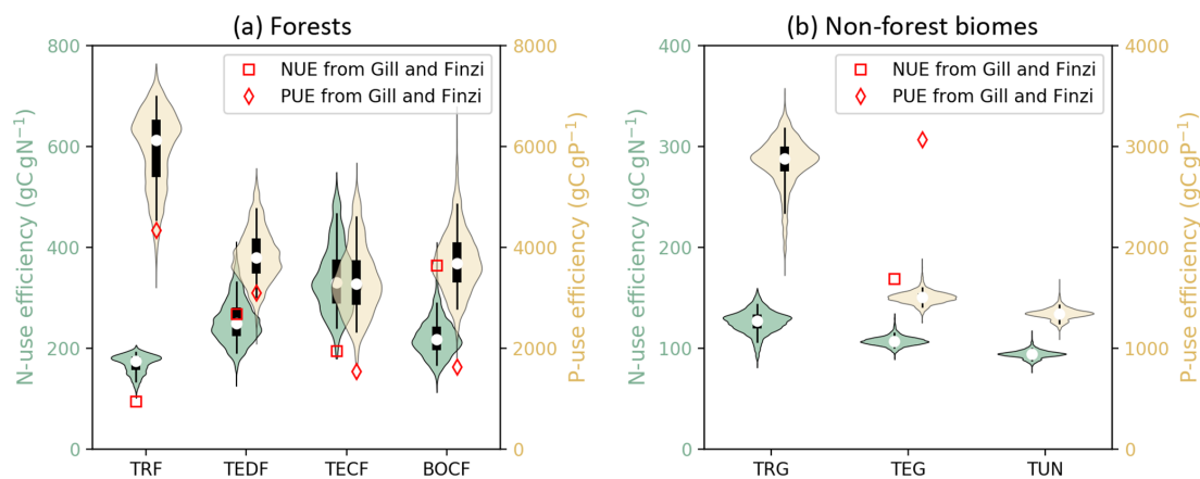
Figure 7. Violin plots of N- and P-use efficiencies (NUE and PUE, the nutrient uptake by plants divided by GPP) of seven biomes. Open circles are medians of all grid cells within each biome, with balloons representing the probability density distribution of each value. Black whiskers indicate the interquartile (thick) and 95 % confidence intervals (thin). (a) Forest biomes, including tropical rainforests (TRF), temperate deciduous (TEDF), temperate coniferous (TECF), and boreal coniferous forests (BOCF). (b) Grassland biomes, including tropical/C 4 (TRG), temperate/C 3 grasslands (TEG), and tundra (TUN). Red squares (NUE) and diamonds (PUE) are the independent estimates from site observations and other generic data sets compiled and harmonized by Gill and Finzi (2016) based on site measurements of GPP and net N/P mineralization.
