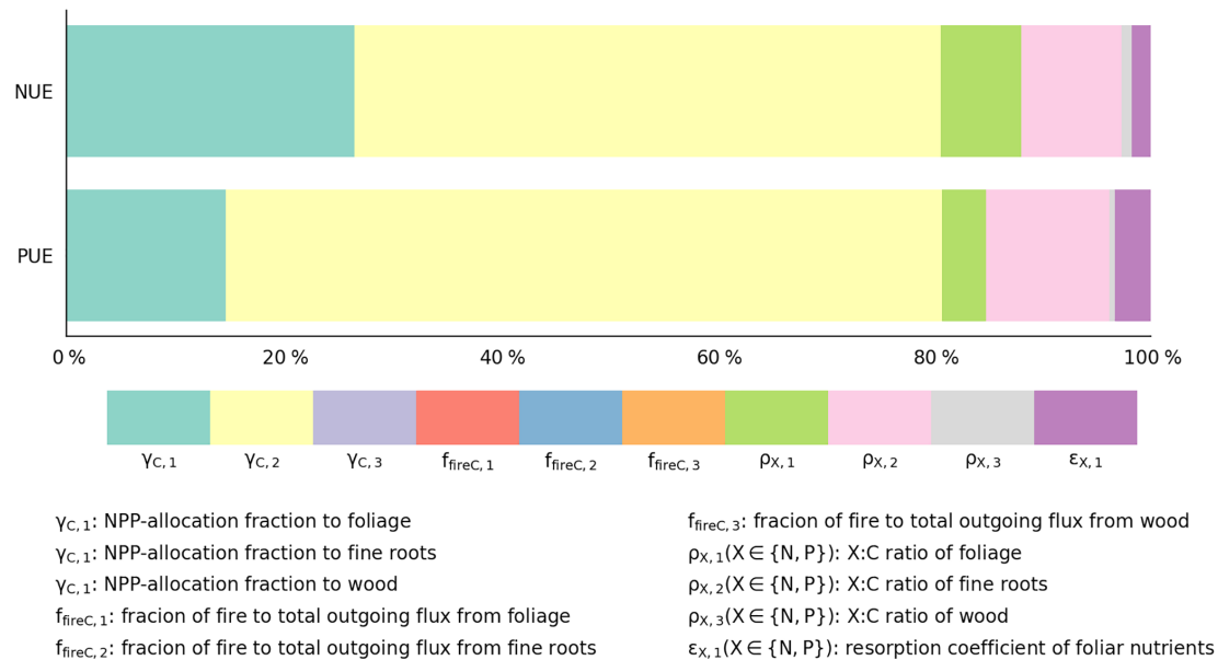
Figure 9. Contribution of input data to the variance in the estimates of nutrient-use efficiencies ( X \in \{N, P\} ) for temperate coniferous forests; \gamma_{C,i=1,2,3} are NPP-allocation fractions to foliage, fine roots, and wood, respectively. f_{\text{fireC},i=1,2,3} are fractions of fire to total outgoing flux from foliage, fine roots, and wood, respectively. \rho_{X,i=1,2,3} ( X \in \{N, P\} ) are X : C ratios of foliage, fine roots, and wood, respectively. \varepsilon_{X,1} ( X \in \{N, P\} ) is the resorption coefficient of foliar nutrients.
