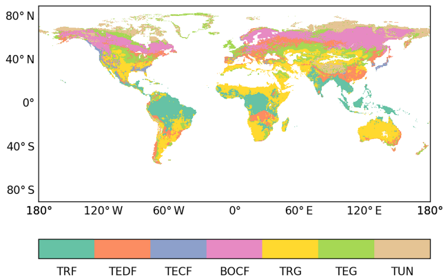
Figure 2. ESA CCI land-cover map classified into the seven large biomes for which average N : C and P : C ratios for each carbon pool are available at a 0.25^\circ \times 0.25^\circ resolution: tropical rainforests (TRF), temperate deciduous forests (TEDF), temperate coniferous forests (TECF), boreal coniferous forests (BOCF), tropical/C 4 grasslands (TRG), temperate/C 3 grasslands (TEG), and tundra (TUN).
