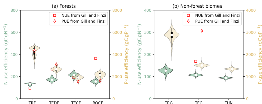
Figure 10. Violin plots of the nutrient-use efficiencies of the seven biomes from the experiment in which the allocation fraction of NPP to woody biomass and to leaves in coniferous forests is reduced. Open circles are the medians of all grid cells within each biome, with balloons representing the probability density distribution of each value. Black whiskers indicate interquartile (thick) and 95 % confidence intervals (thin). The biomes are tropical rainforests (TRF), temperate deciduous forests (TEDF), temperate coniferous forests (TECF), boreal coniferous forests (BOCF), tropical/C 4 grasslands (TRG), temperate/C 3 grasslands (TEG), and tundra (TUN). The red squares (NUE) and diamonds (PUE) are the independent estimates from site observations and other generic data sets compiled and harmonized by Gill and Finzi (2016) based on site measurements of GPP and net N/P mineralization.
