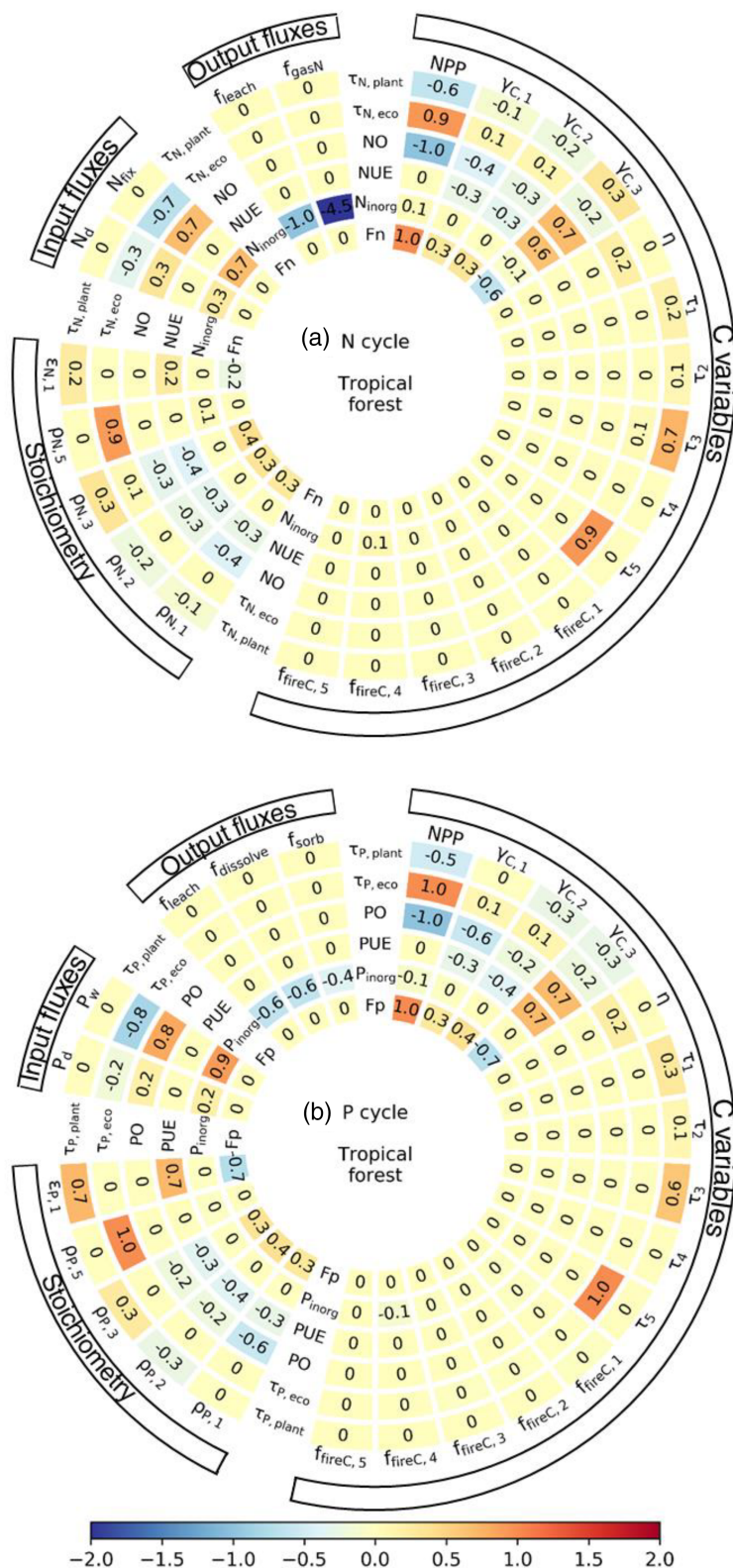
Figure 8. Mean sensitivity of the estimates of rates of nutrient uptake, inorganic nutrients, nutrient-use efficiencies, openness, turnover time of nutrients in the ecosystem, and turnover time of nutrients in plants to the input variables for tropical forest. Results for other biomes are shown in Figs. S7–S12.
