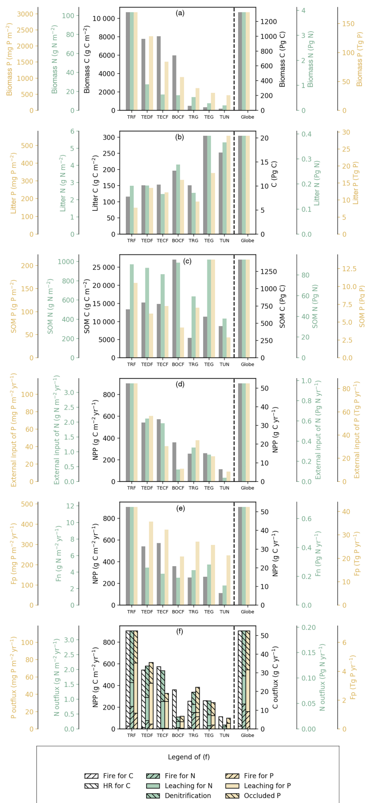
Figure 4. Pool sizes and fluxes of C (black), N (green), and P (yellow) computed from GOLUM-CNP.
