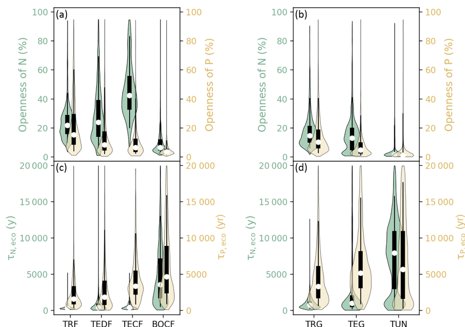
Figure 6. Violin plots of the openness of N and P cycling (the percentage of total plant uptake of N and P attributed to new nutrient inputs) for (a) forest and (b) grassland biomes. Residence times of N ( \tau_{N,eco} ) and P ( \tau_{P,eco} ) in (c) forest ecosystems and (d) grassland biomes. Open circles are medians of all grid cells within each biome, with balloons representing the probability density distribution of each value. Black whiskers indicate the interquartile (thick) and 95 % confidence intervals (thin). The biomes are tropical rainforests (TRF), temperate deciduous forests (TEDF), temperate coniferous forests (TECF), boreal coniferous forests (BOCF), tropical/C 4 grasslands (TRG), temperate/C 3 grasslands (TEG), and tundra (TUN).
