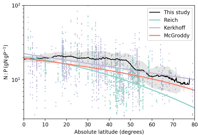
Figure 5. Relationship between foliar N : P ratios ( \text{gN gP}^{-1} ) and absolute latitude. The black line is the mean N : P ratios from this study, and the shaded area is the one-sigma standard deviation of the N : P ratios for a specific latitude. Colored lines are the regression trends of foliar N : P ratios as a function of absolute latitude from Reich and Oleksyn (2004; green), Kerkhoff et al. (2005; blue), and McGroddy et al. (2004; red). Dots are the raw data that Reich and Oleksyn (2004; green) and Kerkhoff et al. (2005; blue) used to derive their regression trends.
