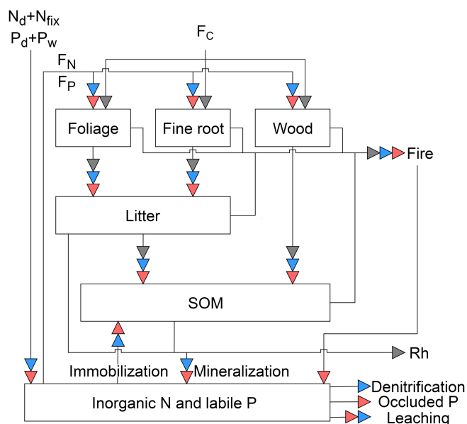
Figure 1. Schematic representation of the pools and fluxes in the C, N, and P cycles within GOLUM-CNP. The gray, blue, and red arrows represent C, N, and P fluxes, respectively. Plants are divided into foliar, fine root, and wood pools, where the wood pool includes woody stems and coarse roots. Litter and soil are two separate pools. The inorganic pool represents the nutrient sources in the soil that are available for plant uptake. Arrows between the pools represent the directions of C, N, and P flow between pools. External inputs of N are atmospheric deposition ( N_d ) and biological N fixation ( N_{fix} ). External inputs of P are atmospheric deposition ( P_d ) and P released by rock weathering ( P_w ). F_C is net primary production (NPP). F_N and F_P are plant uptake of N and P from the inorganic N and labile P pools, respectively. R_h is release of C due to heterotrophic respiration. Mineralization of N and P is modeled along with litter and SOM decomposition, and N and P immobilization is modeled by a flux from the inorganic pool to SOM. External losses of N occur by fire, leaching, and denitrification. External losses of P occur by fire, leaching, and transfer to occluded P in the soil.
