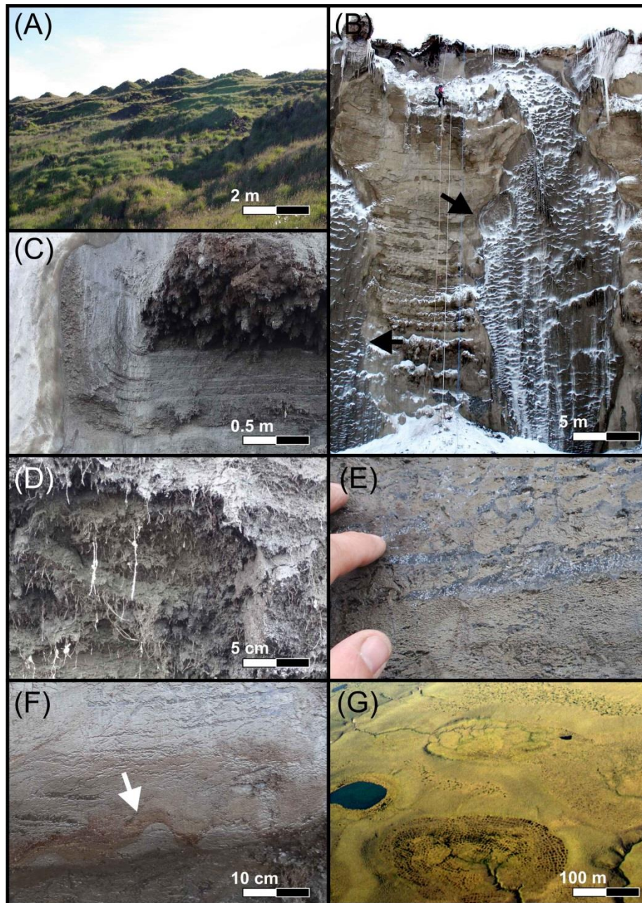
Fig. 3. Typical phenomena of Yedoma deposits and Yedoma landscapes. (A) conical thermokarst mounds (called baidzharakhs in Russia) that developed from sediment-rich polygon centers and the thawing of surrounding large syngenetic ice wedges (Buor Khaya Peninsula, Siberia, 2010) (B) Yedoma bluff, eroded by the Itkillik River (Alaska, 2012). The presence of ice-wedge shoulders (arrows) indicate the position of the paleo active layer and episodic sedimentation of the sediments on the polygonal ground surface; (C) Peat layer and vertically-deformed sediments and ice bands along a syngenetic ice-wedge on Sobo-Sise Island (Lena Delta, Siberia, 2014); (D) Late Pleistocene plant remains (grass roots) in Yedoma deposits on Sobo-Sise Island (2014); (E) Typical cryostructures in Yedoma deposits, here irregular reticulate in the upper part, one ice band in the middle and wavy lenticular in the lower part (photo by D. Fortier, 2012 at Itkillik River exposure, Alaska); (F)
