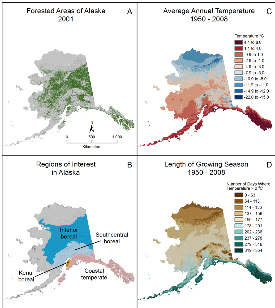
Fig. 1. Alaska maps illustrating (A) total forested area, (B) forest region boundaries of the: (1) Interior-boreal forest that is bounded by the Brooks Range to the north, the Alaska Range to the south, and the Seward Peninsula to the west; (2) Southcentral-boreal forest that includes the forests south of the Alaska Range, west of the Alaska-Yukon border, and east of the Alaska Peninsula; (3) Kenai-boreal forest that includes the western side of the Kenai Peninsula; and (4) Coastal-temperate forest that occurs on the Alaska Panhandle, the eastern portion of the Kenai Peninsula, Prince William Sound, and the islands of the Kodiak archipelago, (C) average annual temperature from 1950–2008, and (D) length of growing season from 1950–2008. Length of growing season values were calculated as the difference between the day of freeze (first Julian date when the temperature was <0^{\circ}\text{C} ) and day of thaw (Julian date when the temperature was >0^{\circ}\text{C} ). The data used to calculate the average annual temperature and length of growing season were obtained from the Climatic Research Unit (CRU; http://www.cru.uea.ac.uk/ ).
