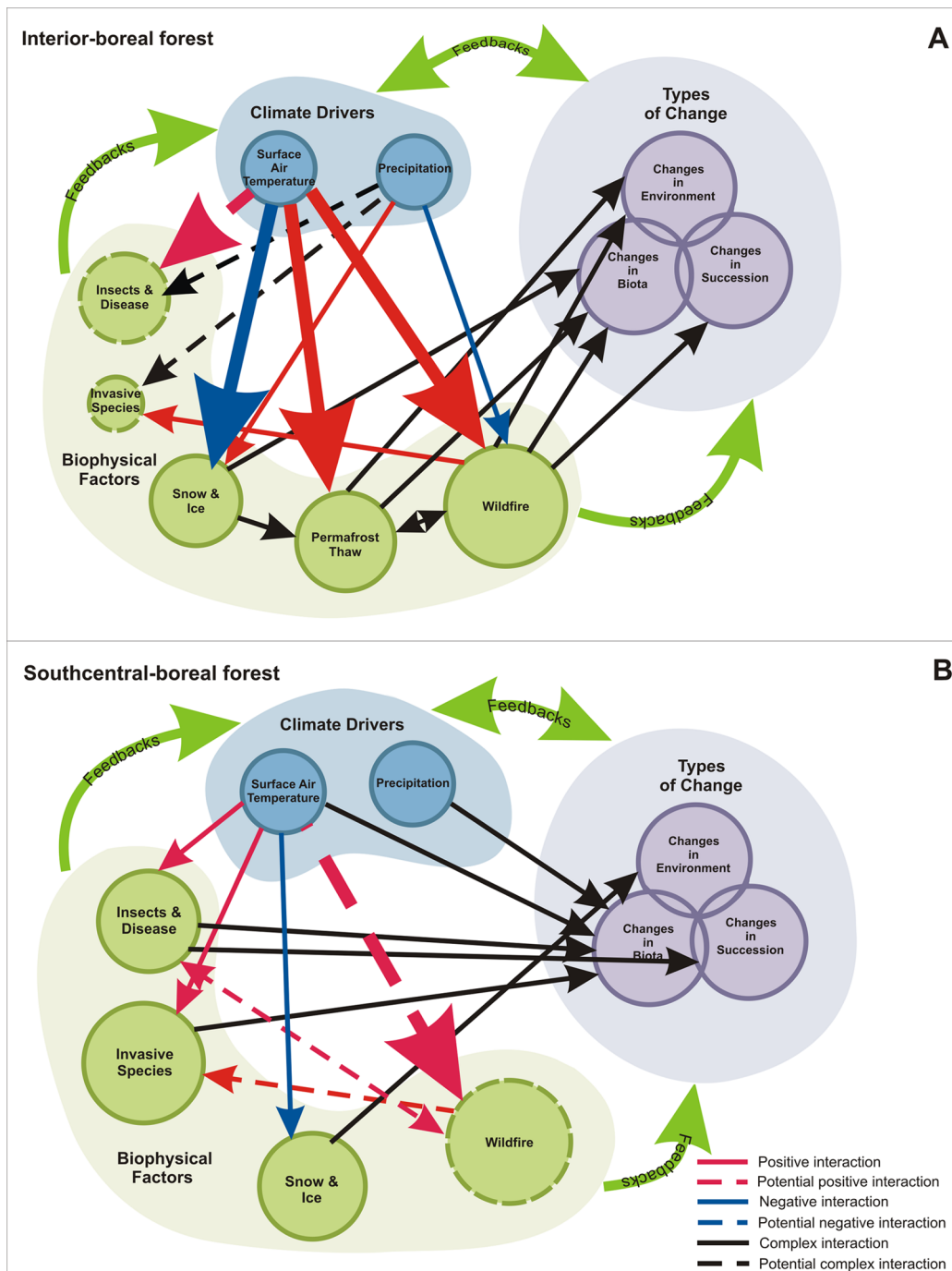
Fig. 3. Regional diagrams of the biophysical subsystem of the conceptual framework (see Fig. 2 and Methods: Creating a framework to evaluate current and future effects of climate change ) depicting climate change impacts in the (A) Interior-boreal; (B) Southcentral-boreal; (C) Kenai-boreal; and (D) Coastal-temperate forest regions of Alaska. Interactions between elements within the biophysical subsystem (defined in Table 1) are supported by research and may be positive (red arrows), negative (blue arrows), or complex (black arrows; i.e., the change in one variable is contingent on the magnitude of change in the other variable).
