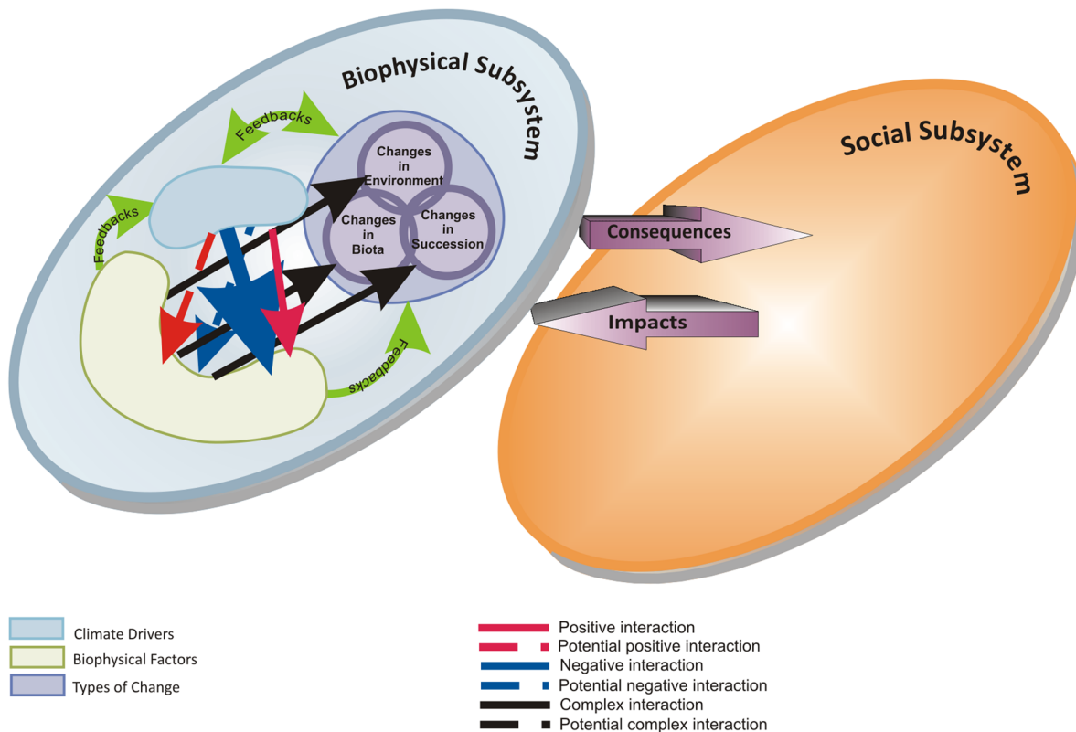
Fig. 2. Conceptual framework of Alaskan forests synthesizing the current understanding of climate-related changes. The framework illustrates the interactions between the biophysical and social subsystems. These subsystems interact via the consequences of ecosystem changes on the social subsystem, and the impacts of the social response to ecosystem changes on the biophysical subsystem. There are interactions (see Fig. 3 for description of arrow color, line type, and thickness) and feedbacks (green labeled arrows) that link the elements of the biophysical subsystem: climate drivers (blue circles), biophysical factors (green circles) and types of change (violet circles) (described in Table 1). The complex interactions occurring between the categories of the types of change (changes in environment, succession and biota) are depicted with overlapping circles.
