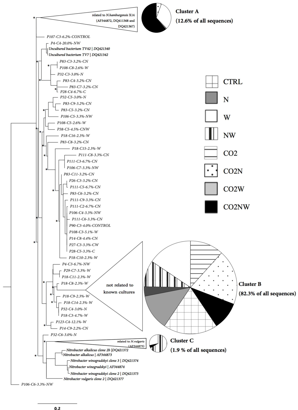
FIGURE 2 | Phylogenetic tree of Nitrobacter -like nxrA sequences retrieved from soils experiencing different global change treatments in relation to nxrA sequences of cultivated strains. Disks represent the distribution of nxrA sequences among treatments for the three main clusters identified (Unifrac Significance for each: p < 0.001 ). These three clusters correspond to 96.8% of all the nxrA sequences retrieved across treatments and to more than 86% of nxrA sequences retrieved for each treatment.
