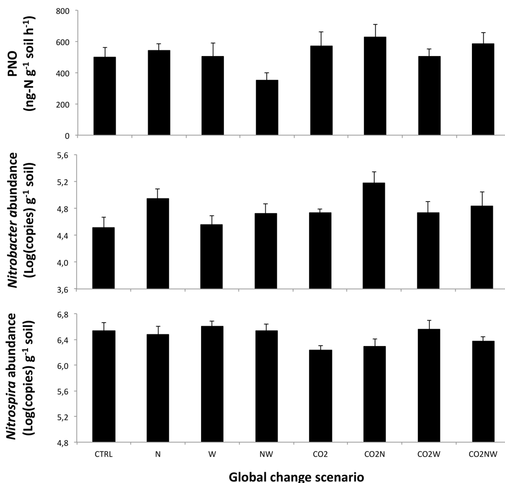
FIGURE 1 | Observed responses of (Top) potential nitrite oxidation, PNO, (Middle) the abundance of total Nitrobacter -like NOB, and (Bottom) the abundance of Nitrospira in response to the different global change scenarios in April 2005. Means are presented with standard errors ( n = 6 ). N, W and CO 2 refer to nitrogen addition, increased precipitation, and elevated atmospheric CO 2 , respectively. CTRL refers to the control treatment where all factors are at ambient levels. Results of statistical analyses of treatment effects are presented in Table 1 .
