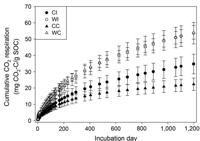
FIGURE 1 Cumulative CO 2 respiration of soils from the four field treatments over the 3-year laboratory incubation. CI: control + intact soil; WI: warm + intact soil; CC: control + collar soil; WC: warm + collar soil. Data are mean ± SE (n = 6)
