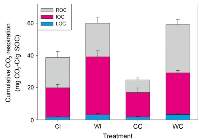
FIGURE 2 Cumulative CO 2 respiration from the decomposition of SOC components in the four treatments after the 3-year incubation. LOC: labile SOC; IOC: intermediate SOC; ROC: resistant SOC. CI: control + intact soil; WI: warm + intact soil; CC: control + collar soil; WC: warm + collar soil. Bars are mean ± SE (n = 6) [Colour figure can be viewed at wileyonlinelibrary.com]
