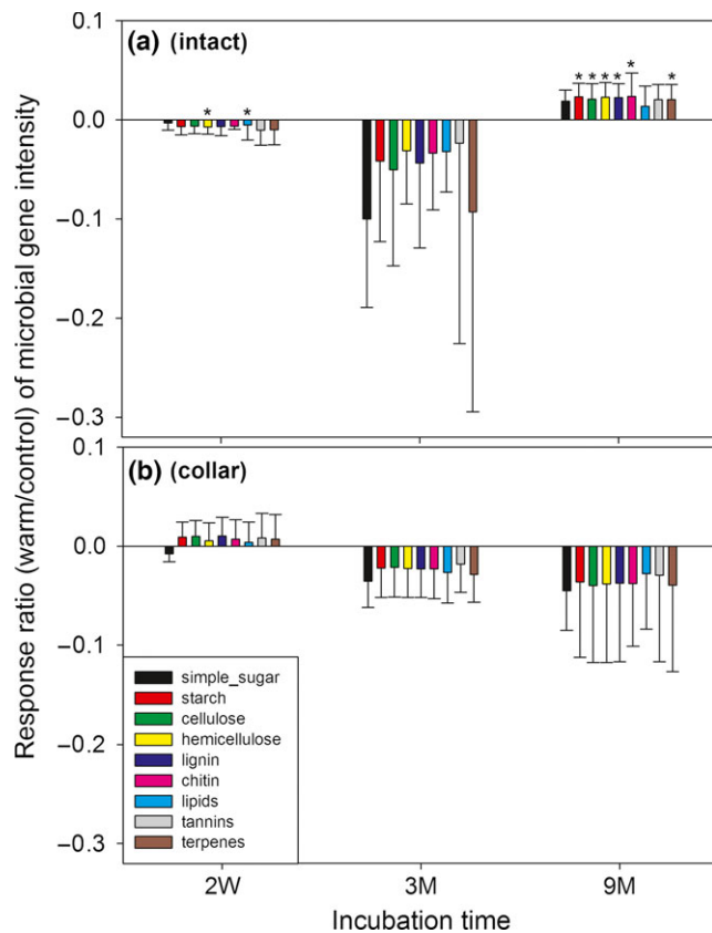
FIGURE 5 The response ratio of signal intensities of microbial genes for the degradation of various organic compounds to warming in intact soils (a) and deep collar (b) soils over the 3-year incubation. 2W, 3M, and 9M are two weeks, three months, and nine months after the laboratory incubation. *represents p < .05
