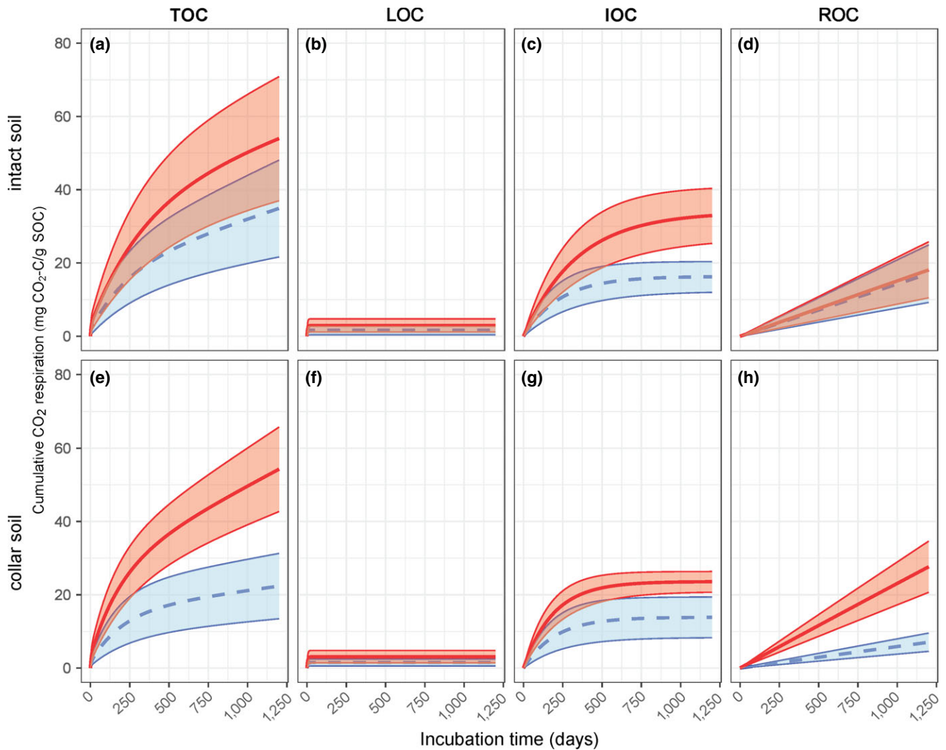
FIGURE 3 Modeled cumulative CO 2 respiration from the decomposition of SOC components of the intact (a–d) and the deep collar soils (e–h) over the 3-year incubation. LOC: labile SOC; IOC: intermediate SOC; ROC: resistant SOC; TOC: total SOC. Red lines refer to field warming, and blue lines refer to the control. Shade areas refer to 95% confidence interval
