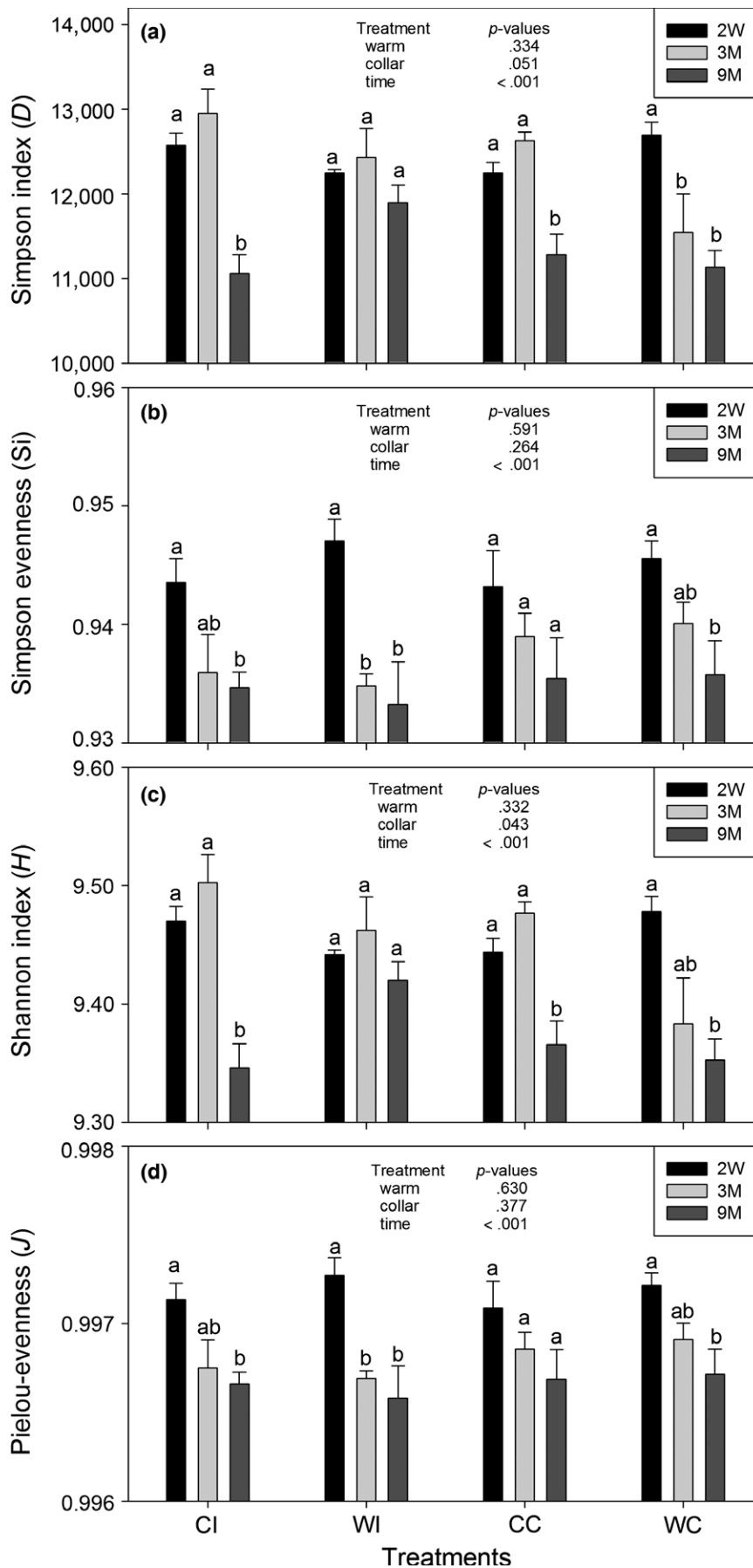
FIGURE 4 Diversity (a–d) of C-degradation microbial genes estimated two weeks (2W), three months (3M), and nine months (9M) after incubation in the four treatments. CI: control + intact soil; WI: warm + intact soil; CC: control + collar soil; WC: warm + collar soil. Different letters mean statistical difference among the three times in each treatment
