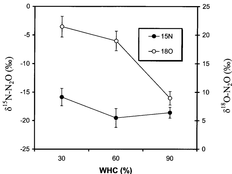
FIGURE 4 Effects of soil moisture content on \delta^{15}\text{N} and \delta^{18}\text{O} (‰).
