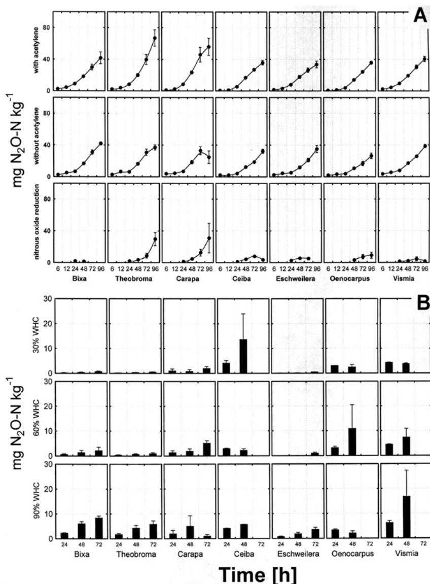
FIGURE 1 (A) Net \text{N}_2\text{O} production ( \text{mg N}_2\text{O-N kg}^{-1} ) during anaerobic incubation in the presence and absence of \text{C}_2\text{H}_2 , and \text{N}_2\text{O} reduction activity (calculated as the difference between \text{N}_2\text{O} concentration with and without \text{C}_2\text{H}_2 ). The symbols indicate means \pm standard errors ( n = 3 ). (B) Net \text{N}_2\text{O} production ( \text{mg N}_2\text{O-N kg}^{-1} ) of soils beneath different tree species in Brazilian Amazon during aerobic incubation under three soil moisture levels (means and standard errors; n = 3 ).
