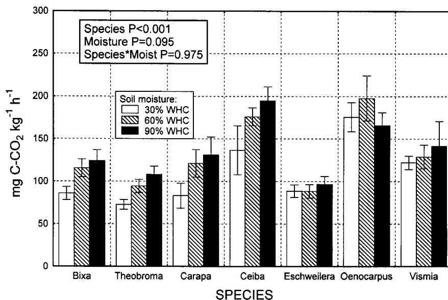
FIGURE 2 The rate of CO 2 production (mg CO 2 -C kg -1 h -1 ) in soils beneath different tree species in the Brazilian Amazon during aerobic incubation under three soil moisture levels. Values are means ± standard errors ( n = 3 )
