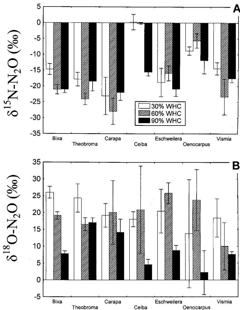
FIGURE 3 \delta^{15}\text{N} (A) and \delta^{18}\text{O} (B) in \text{N}_2\text{O} (‰) produced by soils beneath different tree species in Brazilian Amazon during aerobic incubation at three soil moisture levels. Values are means \pm standard errors ( n=3 )
